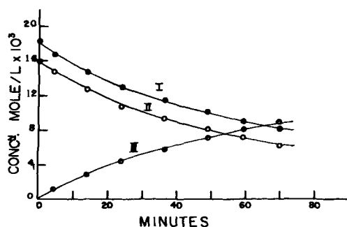
Fig. 4.—Rate of photoreduction of benzophenone by benzhydrol in KBr: I, disappearance of benzophenone; II, disappearance of benzhydrol; III, formation of benzopinacol.
